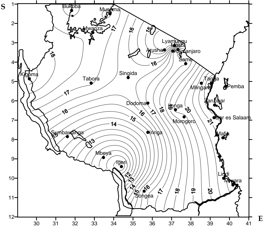
Figure 3: Mean annual minimum temperature (°C)
